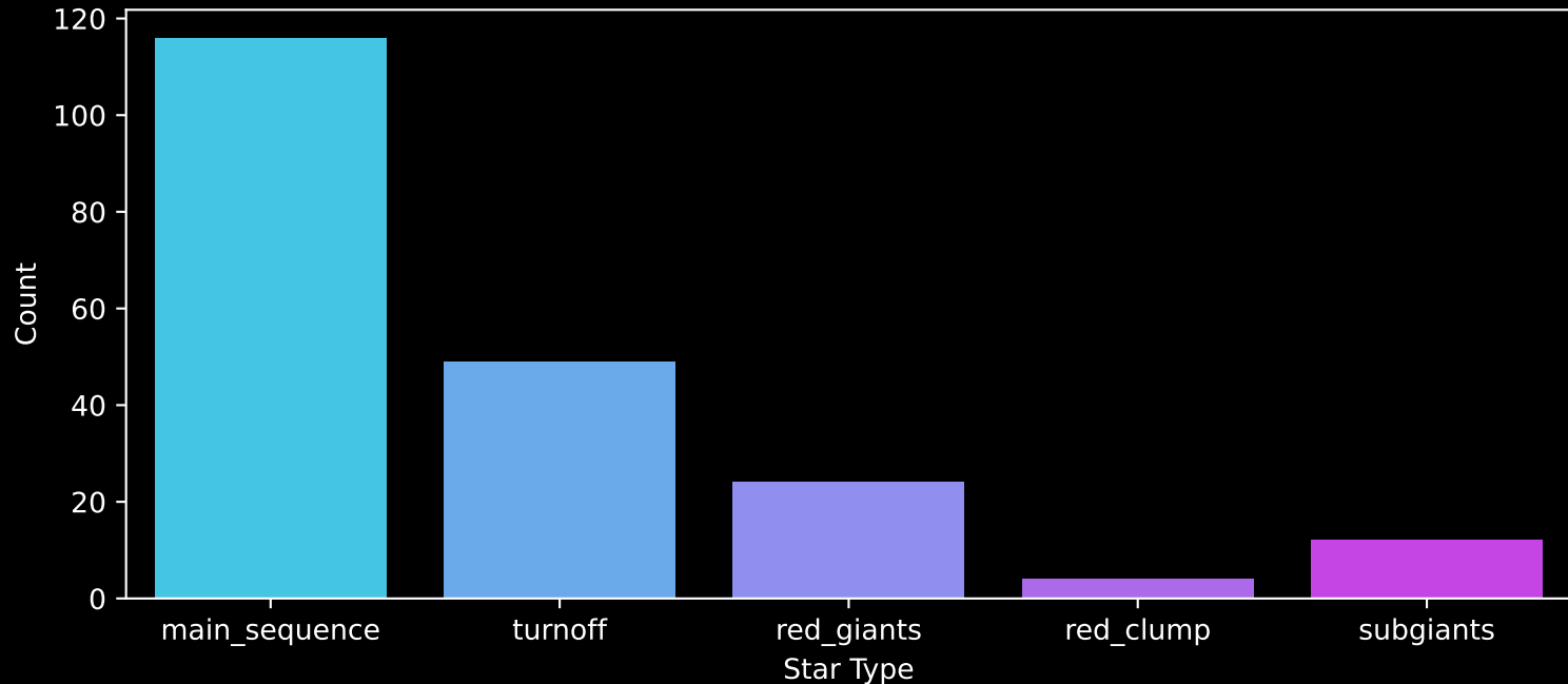
APOGEE DR17 Field: [K2EB_C06_327+54_btx] Count plot of Star Type
