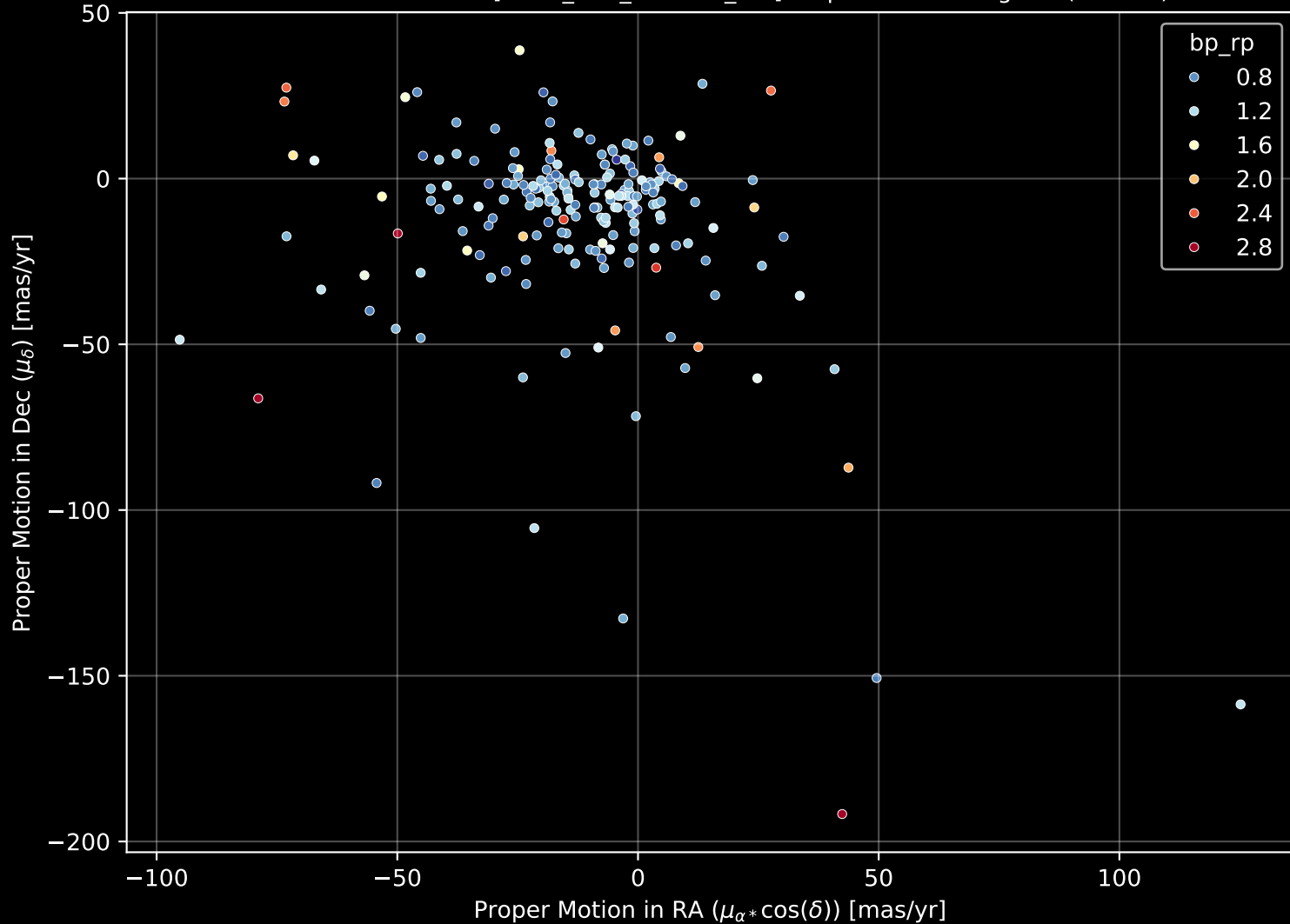
APOGEE DR17 Field: [K2EB_C06_327+54_btx] Proper Motion Diagram (n= 205)
