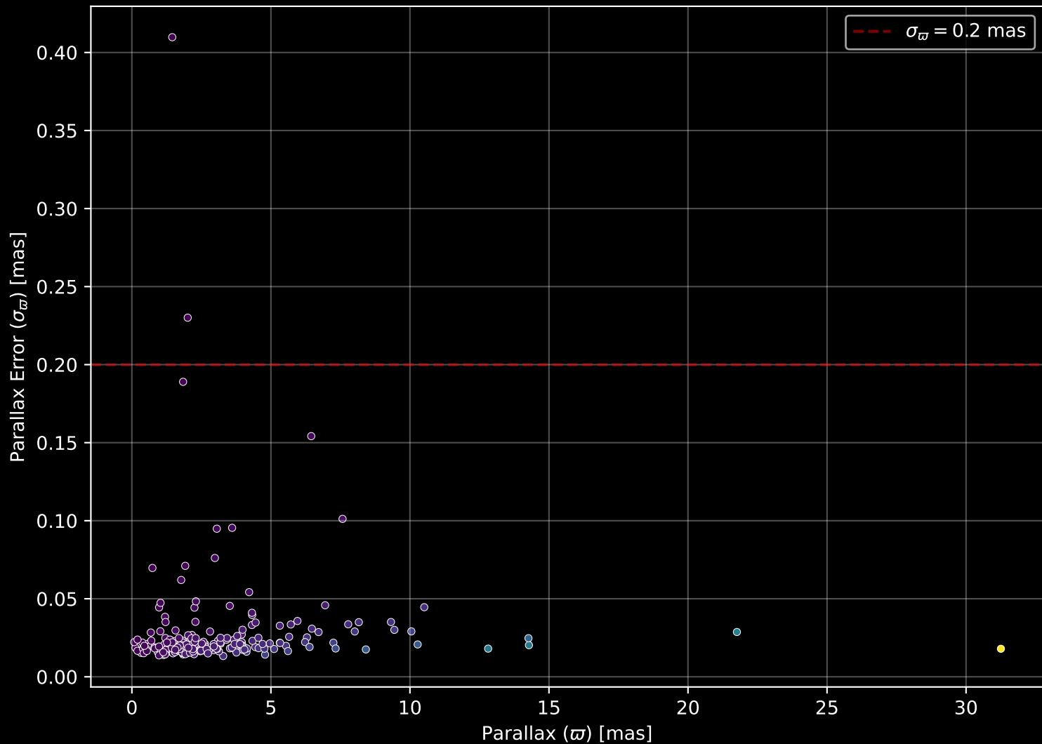
APOGEE DR17 Field: [K2EB_C06_327+54_btx] Parallax Quality (n= 205)
