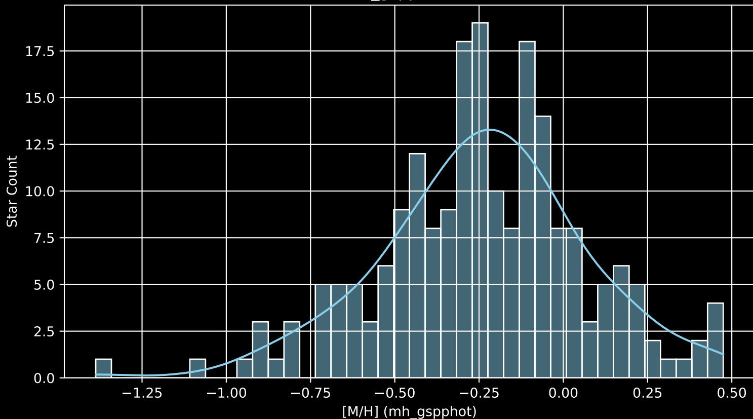
APOGEE DR17 Field: [K2EB_C06_327+54_btx [M/H] (mh_gspphot) (n= 204)
