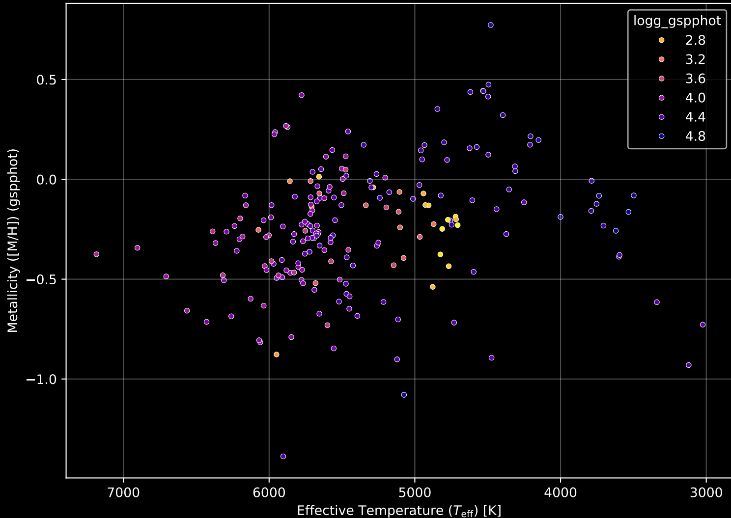
APOGEE DR17 Field: [K2EB_C06_327+54_btx] Stellar Population Parameters (n= 205)
