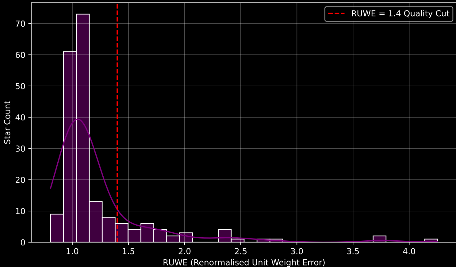
GAPOGEE DR17 Field [K2EB_C06_327+54_btx] RUWE Distribution (n= 199)
